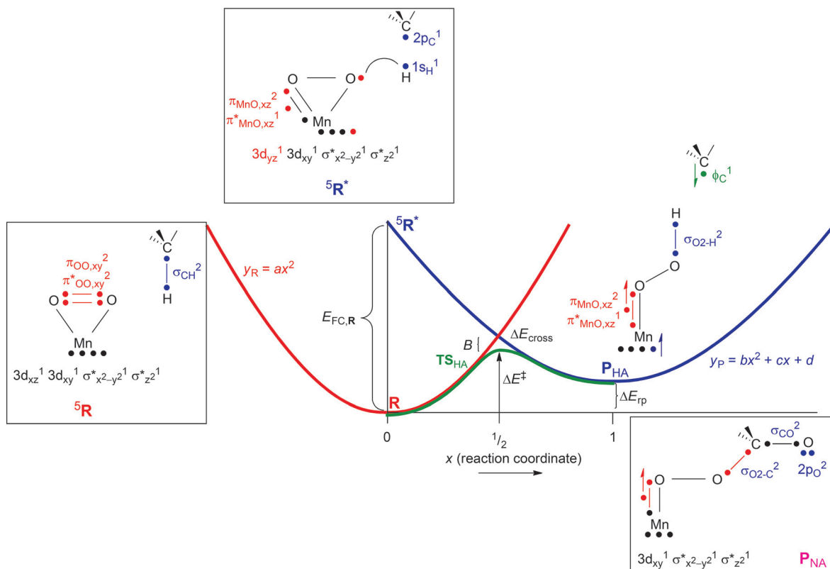
Figure 3. Two-parabola curve-crossing rationalization of the hydrogen-atom abstraction pathway in the reaction of 1 with 2-PPA. Bond orbital changes along the pathways highlighted. Dots represent electrons, and a line between two dots is a bond occupied by two electrons. Straight arrows indicate spin orbitals. Also shown is the VB representation of the alternative nucleophilic intermediate P NA .
